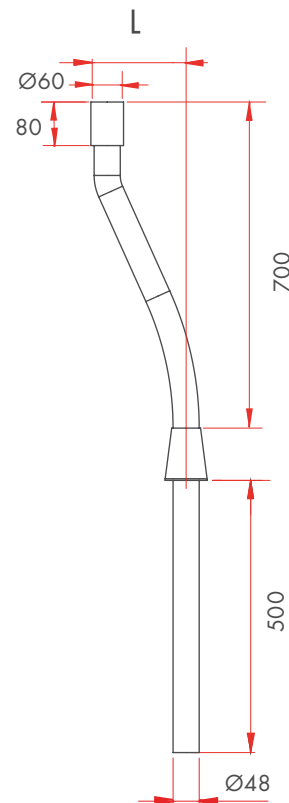
• ELBO SINGLE LIGHT
