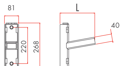
• KEALIT WALL AND OFFSET 200
