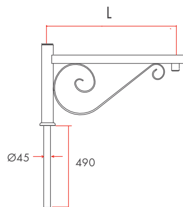
• VÉRONÉ SINGLE LIGHT
