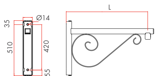
• VÉRONÉ WALL AND OFFSET LIGHTS
